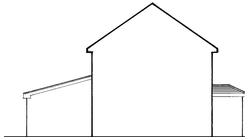
Proposed North/ Side Elevation
