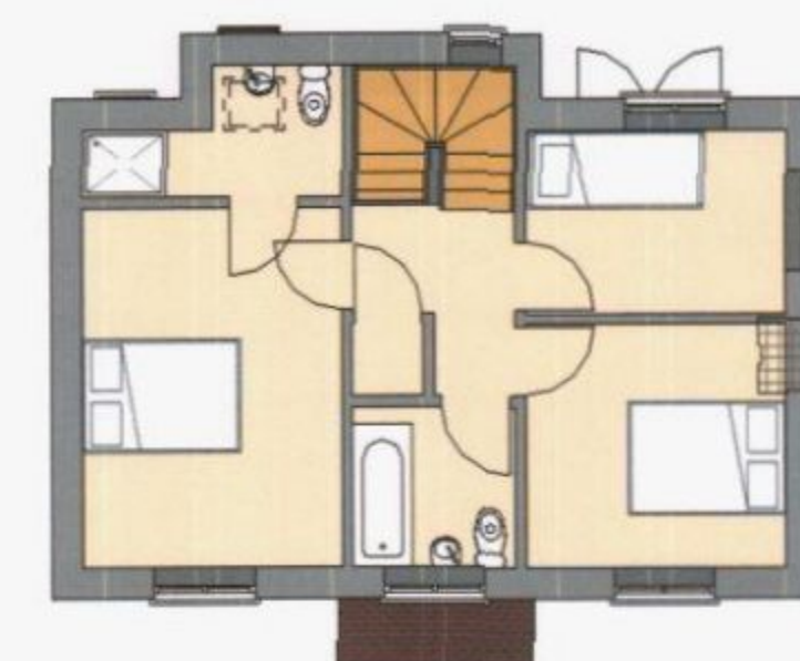
Type 26- Plot 79 First Floor 1 : 100
