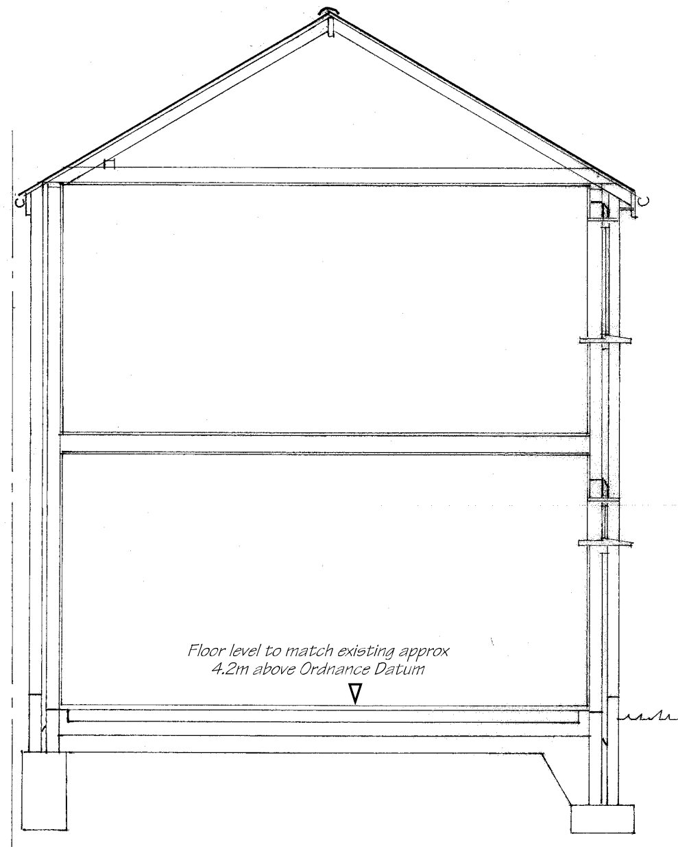
Cross-Section
