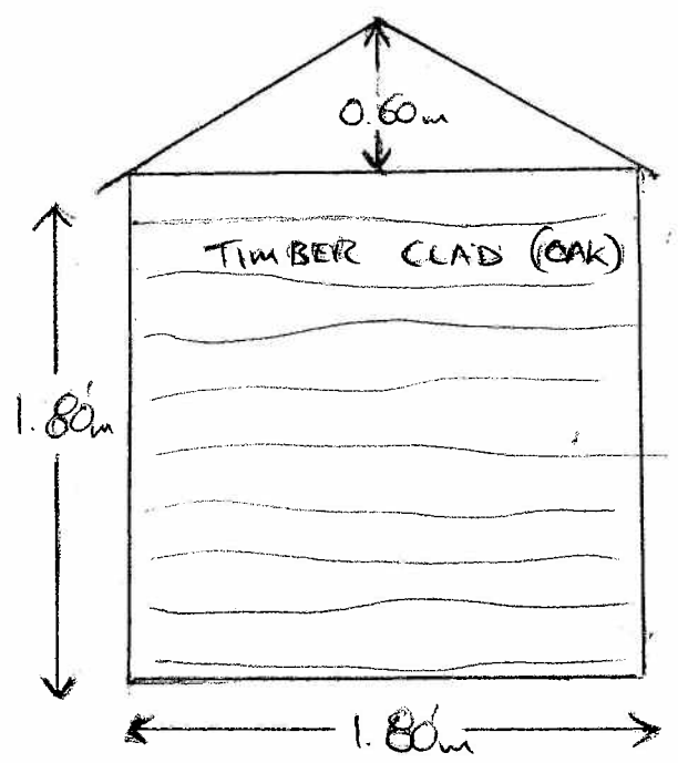
SOUTH ELEVATION
