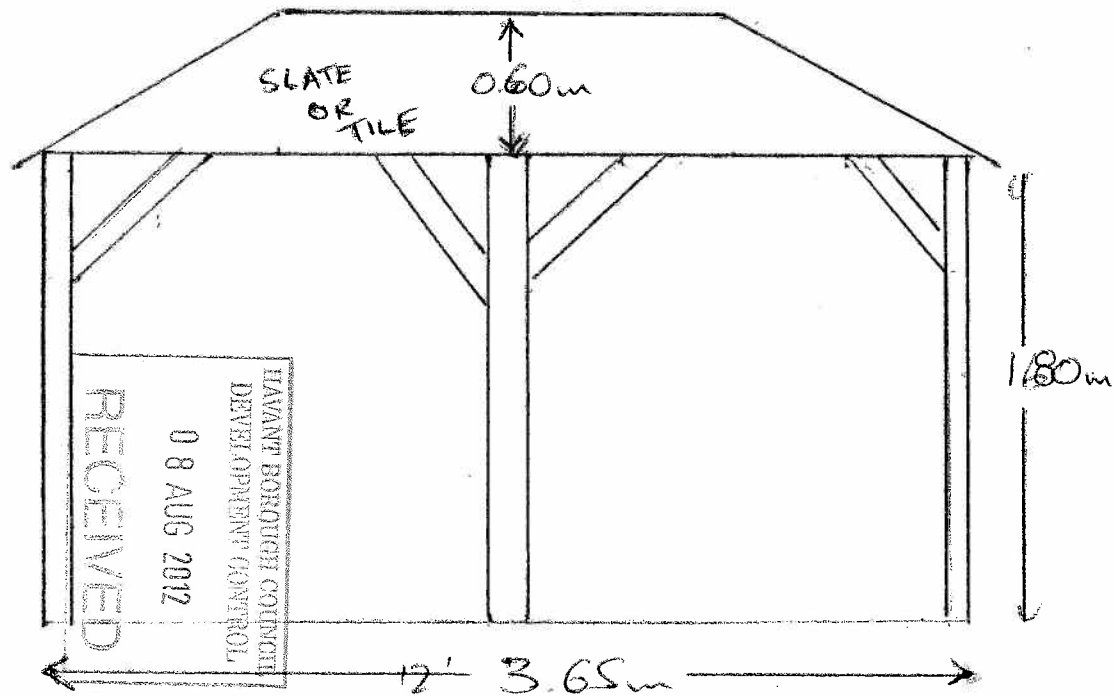
EAST ELEVATION
