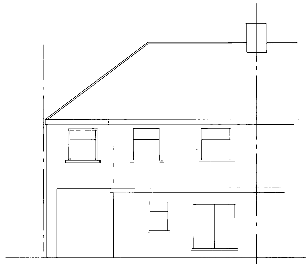
Existing West/Rear Elevation
