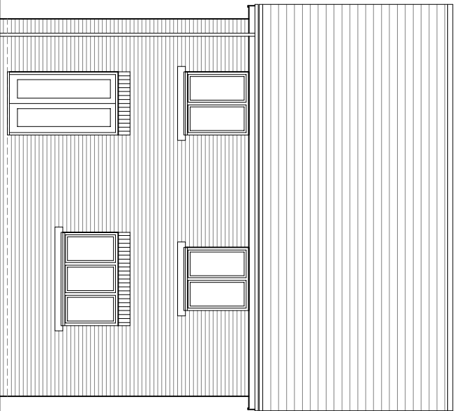
Rear Elevation
