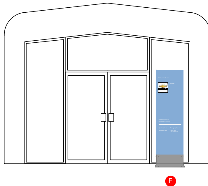
ELEVATION A SCALE 1:50
