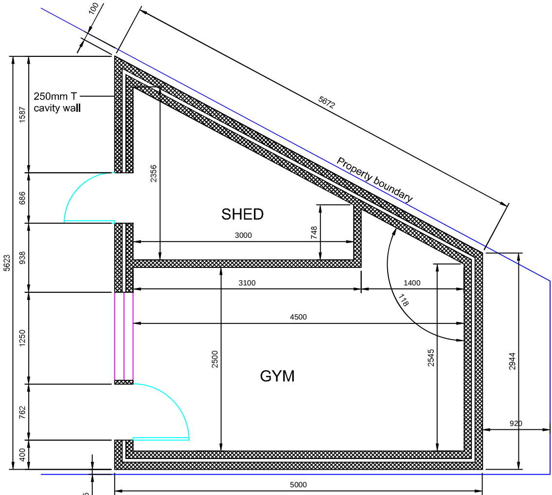
OUTBUILDING PROPOSED
