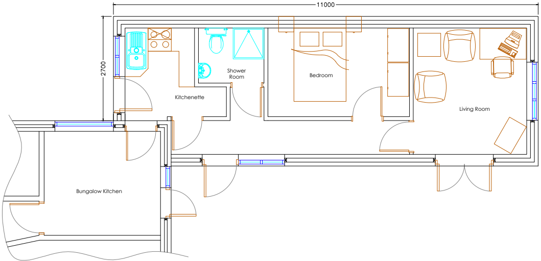
Proposed Floor Layout
