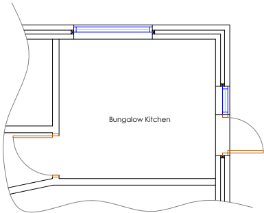
Existing Floor Layout
