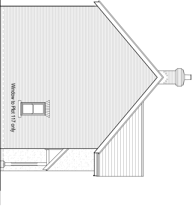
Side Elevation
