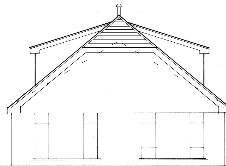
Proposed NE/Front Elevation
