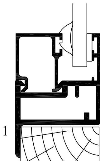
SERIES 40 6mm SQUARE BEAD OPTION
