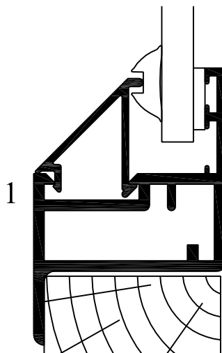
SERIES 40 6mm CHAMFER BEAD OPTION
