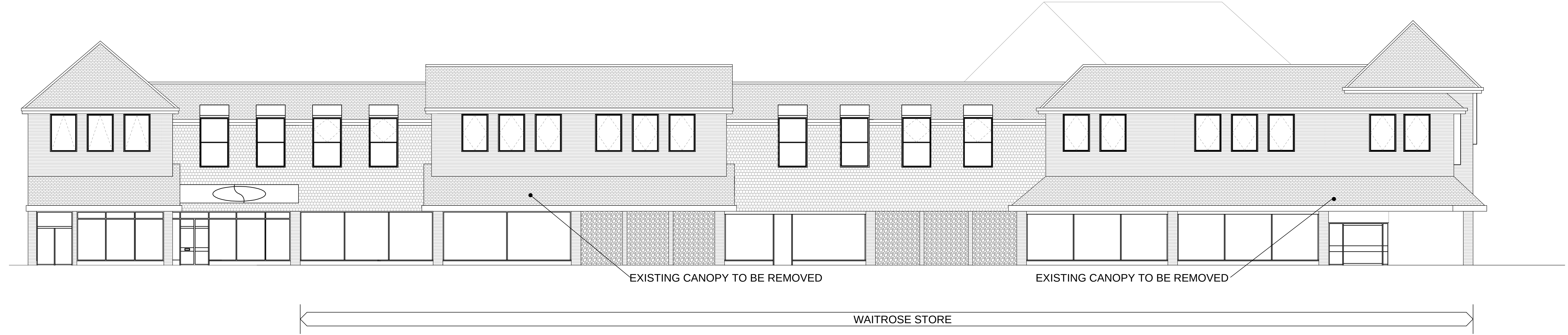
ELEVATION TO NORTH STREET
