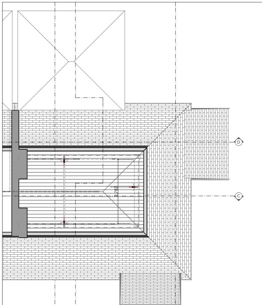
Existing Loft Plan 1:100
