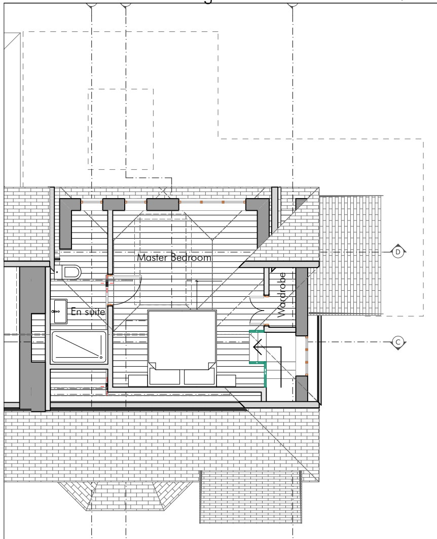
Proposed Loft plan 1:100
