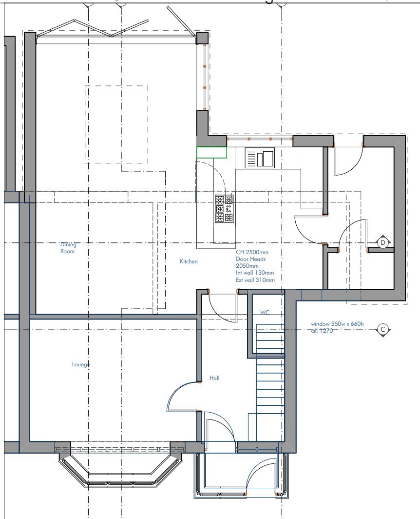
Ground Floor Proposed Plan 1:100
