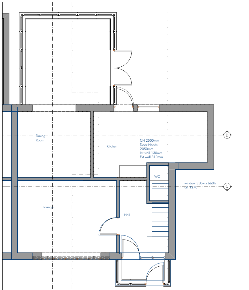
Ground Floor Existing Plan 1:100
