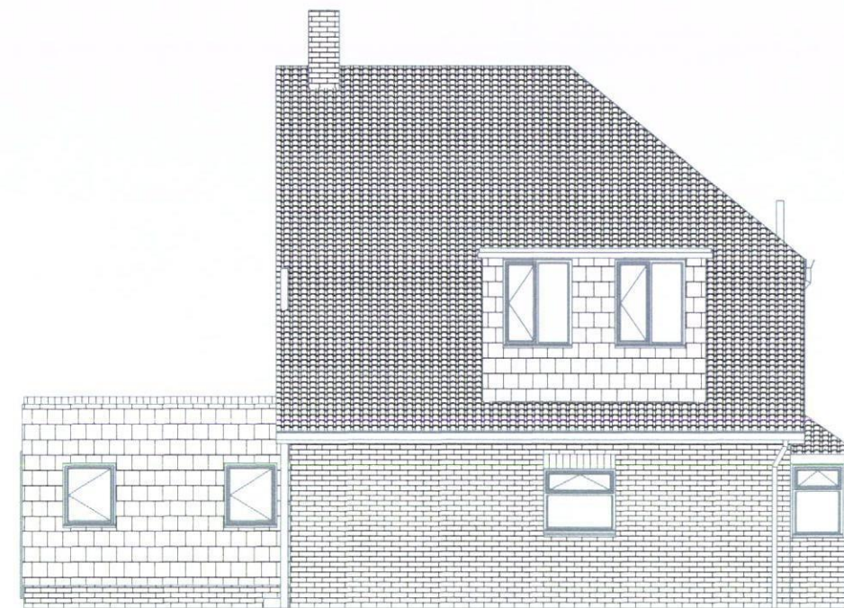
2 ELEVATION SOUTH EAST 1 : 100
