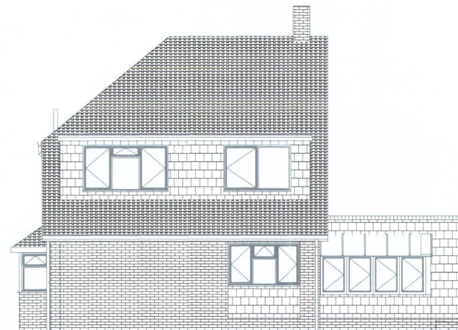
4 ELEVATION NORTH WEST 1 : 100
