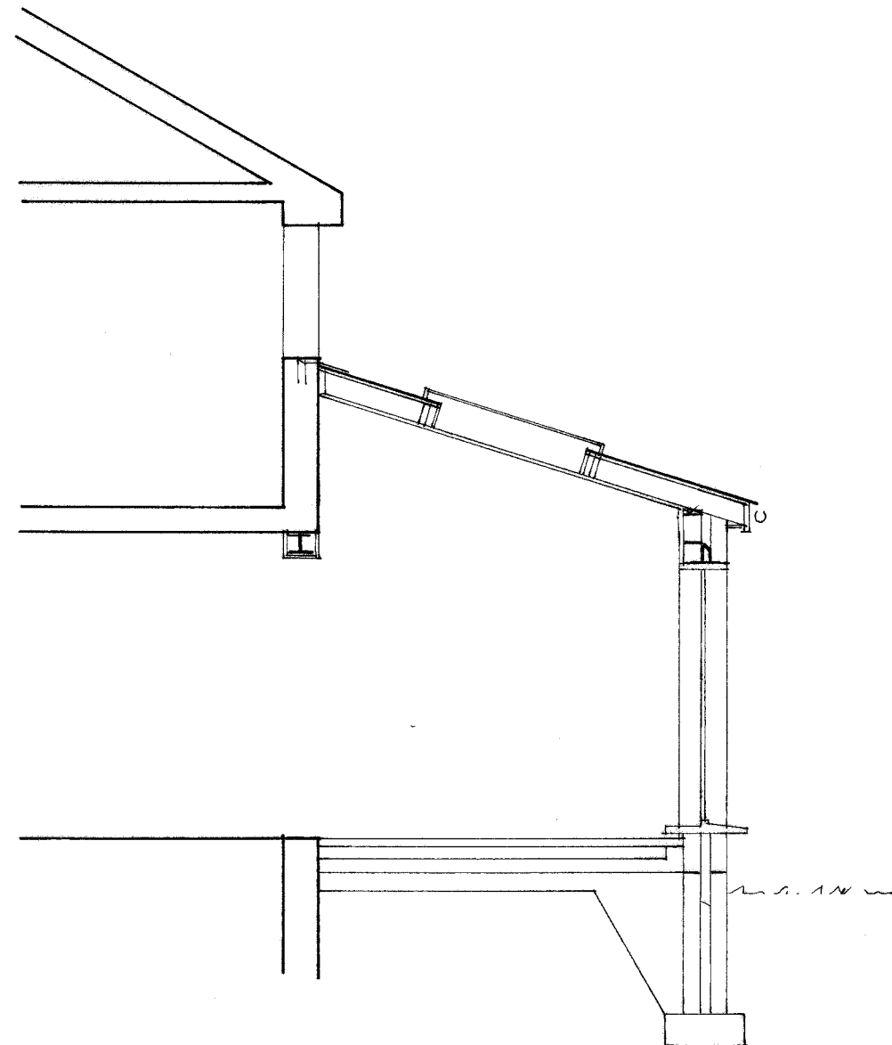
Cross-Section
