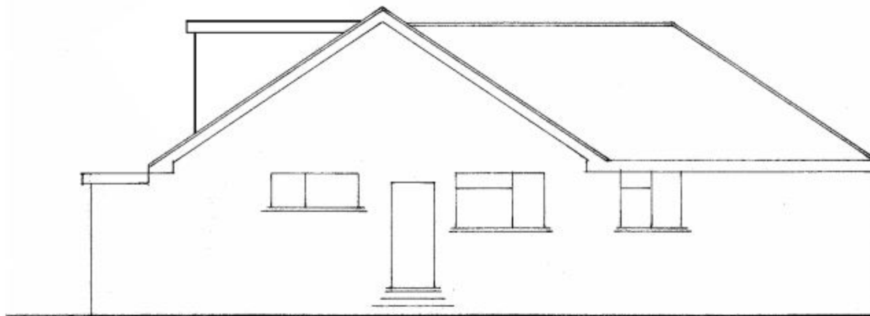
Proposed Side Elevation (Other Dormer /Side Elevation Handed)
