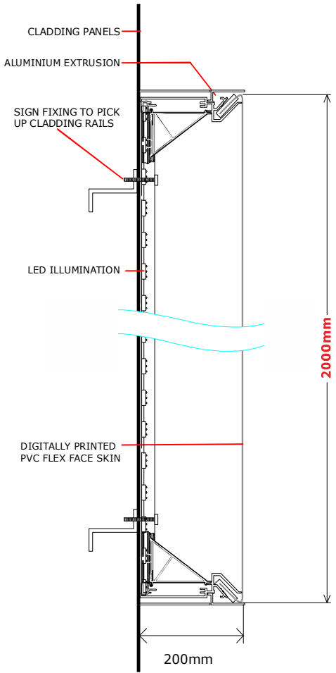
FLEXFACE SECTION THROUGH 1:10
