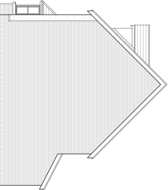
Side Elevation
