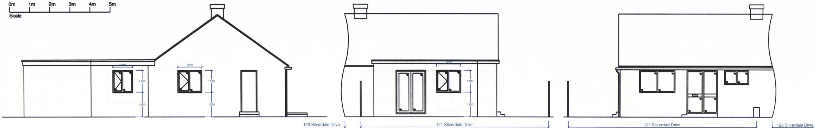
Proposed South West Elevation
