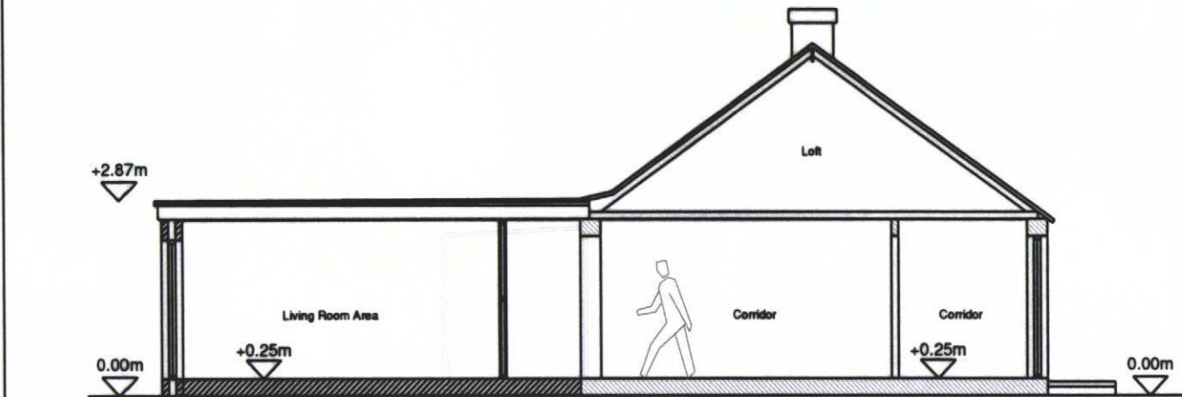
Proposed Cross Section Through A-A
