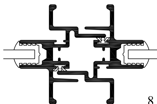
BUTT INTERLOCK
