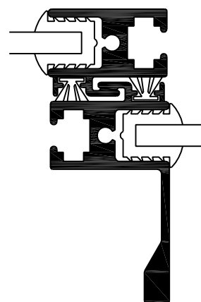
REVERSE INTERLOCK
