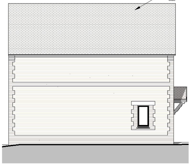
Type 5- Plot 11 Left elevation 1 : 100
