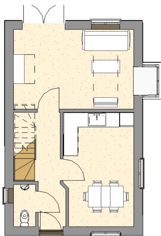
Type 5- Plots 11 Ground Floor 1 : 100
