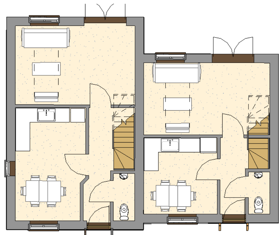
Type 6- Plots 55, 56 Ground Floor 1 : 100
