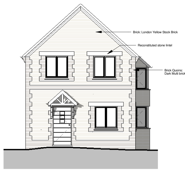
Type 5- Plot 11 Front elevation 1 : 100
