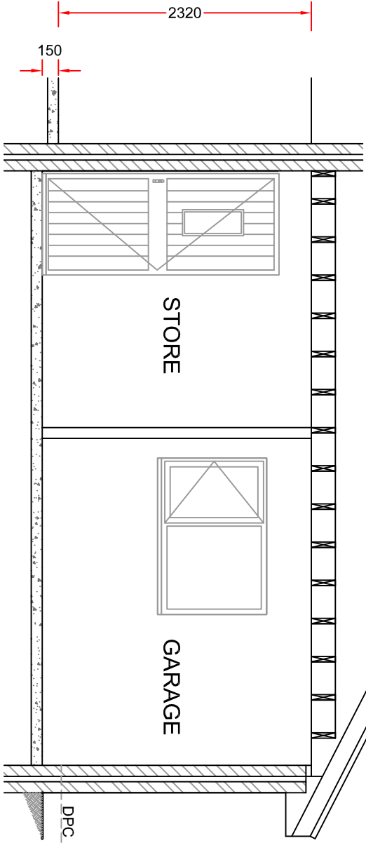
EXISTING SECTION A-A
