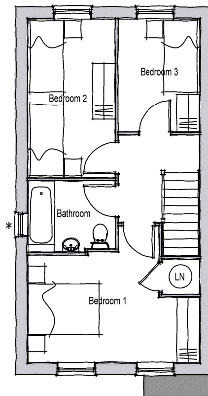
FIRST FLOOR PLAN * WINDOW TO PLOTS 70 & 71 ONLY
