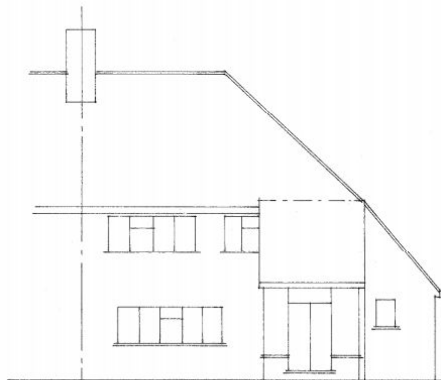
Existing South/Front Elevation
