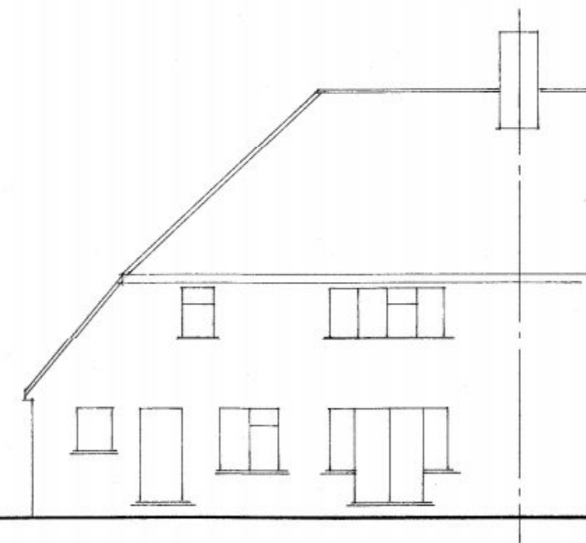
Existing North/Rear Elevation
