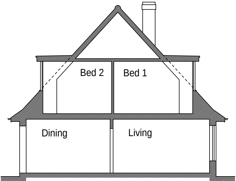
Existing Section A-A
