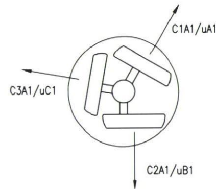
ANTENNA PLAN
