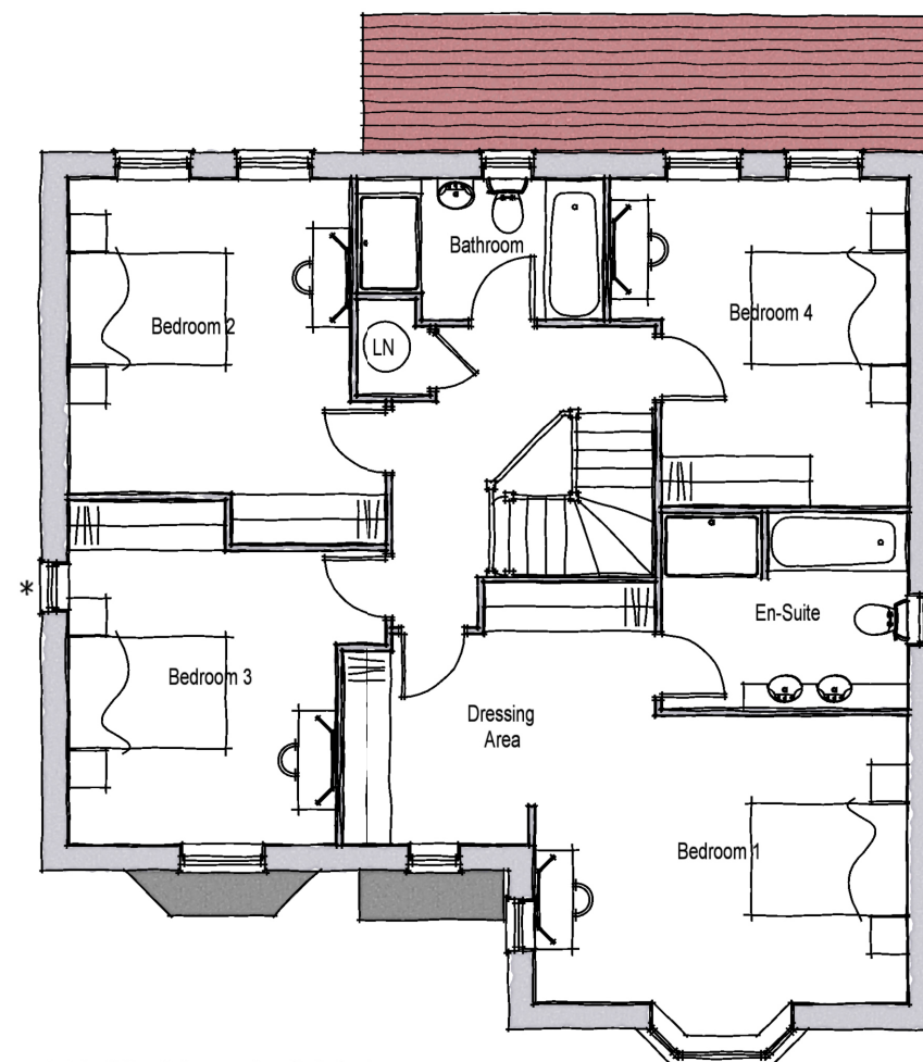
FIRST FLOOR PLAN * PLOT 6 ONLY
