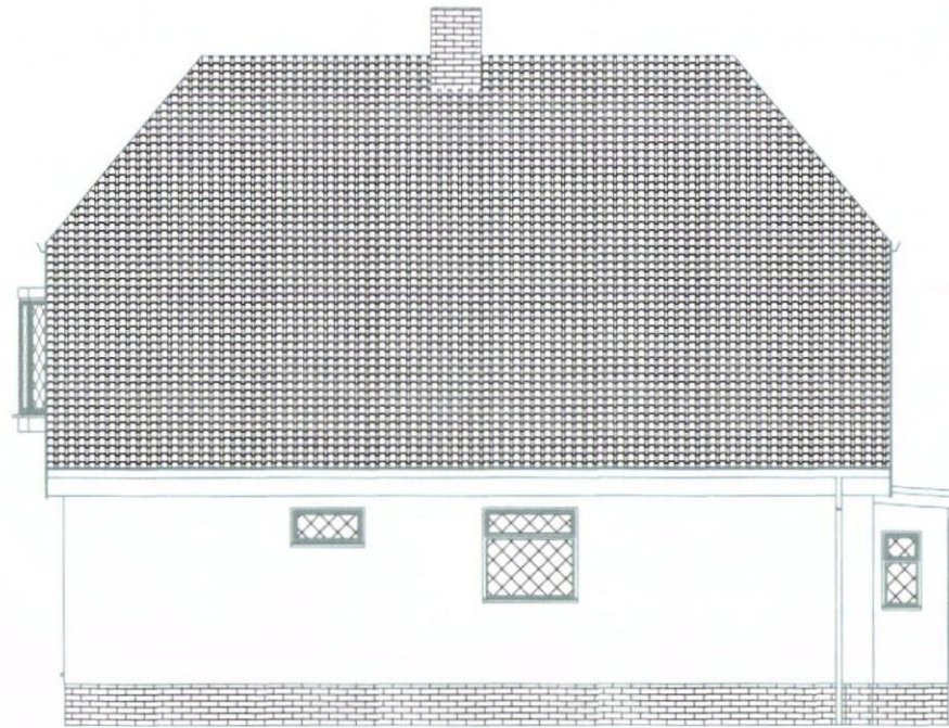
2 EXISTING ELEVATION REAR (SW)
