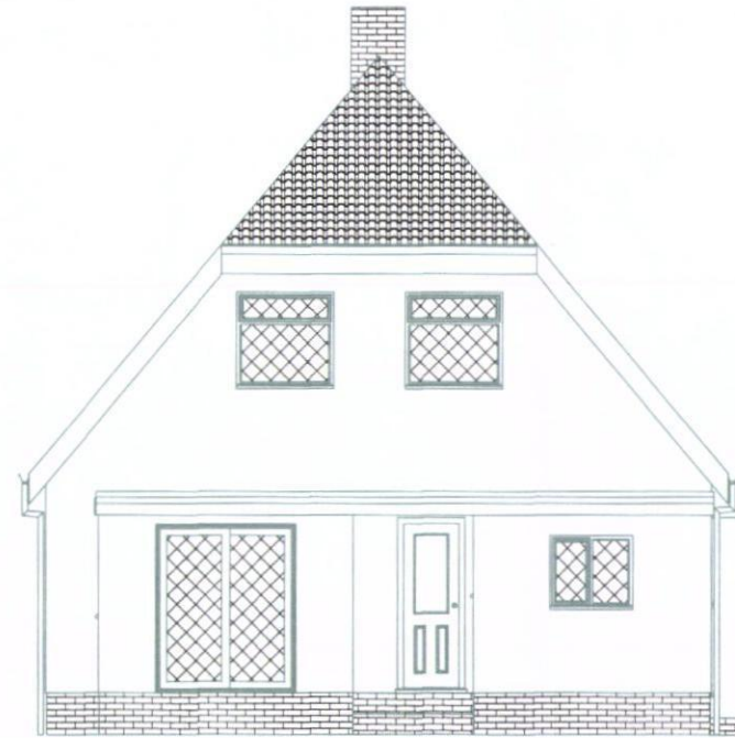
4 EXISTING ELEVATION SIDE (SE)
