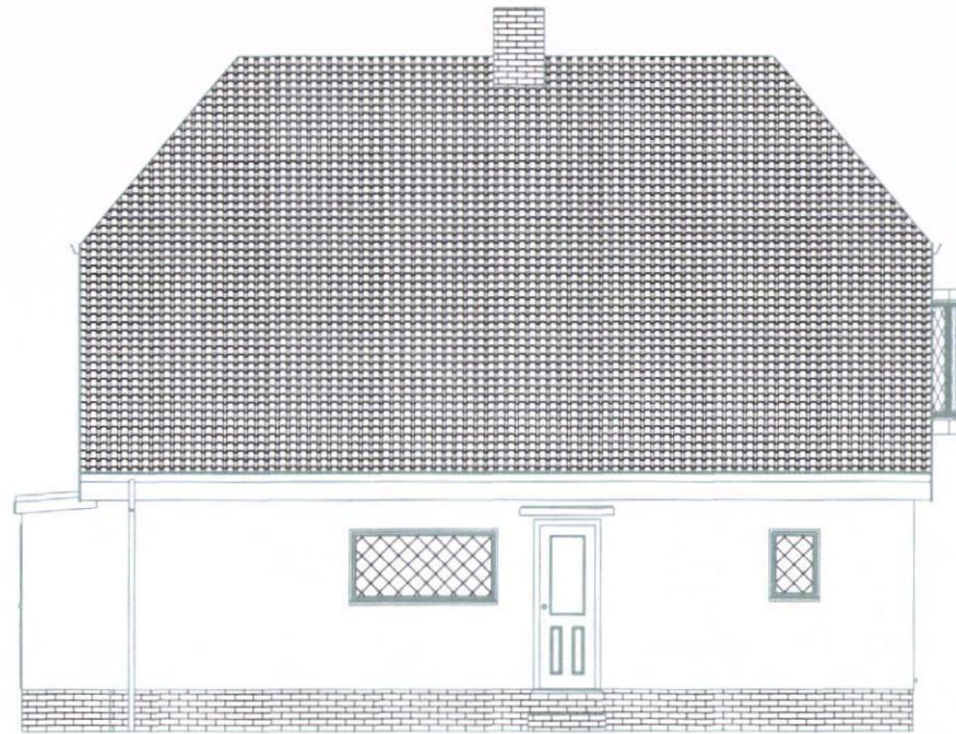
1 EXISTING ELEVATION FRONT (NE)
