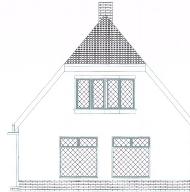
3 EXISTING ELEVATION SIDE (NW)
