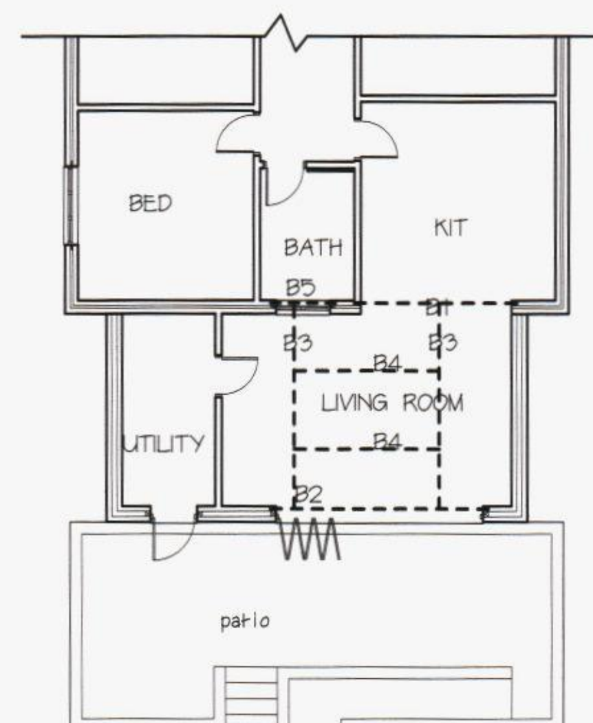
PLAN
