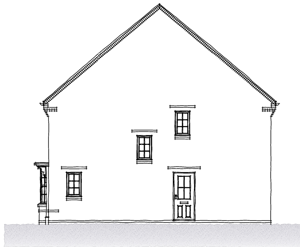
SIDE ELEVATION
