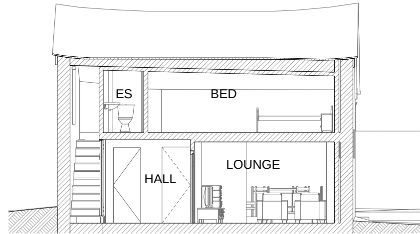
LONG SECTION LOOKING TO NORTH: AS PROPOSED
