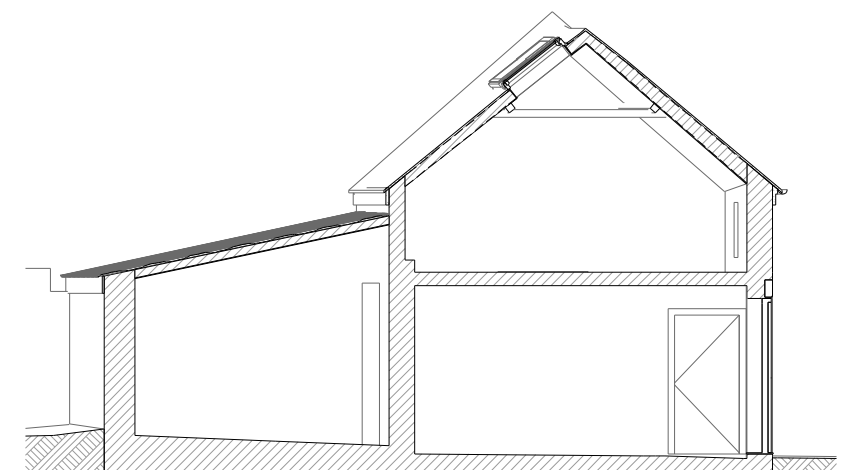
CROSS SECTION LOOKING TO EAST: AS EXISTING
