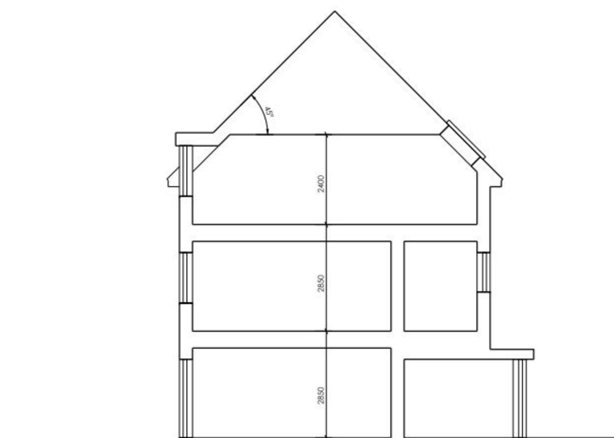
SECTION C-C
