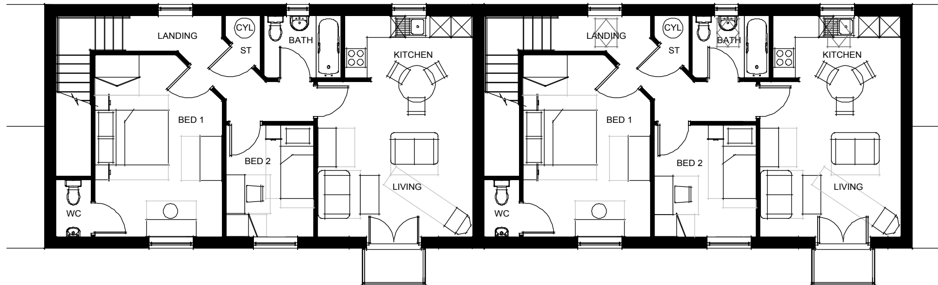
First Floor
