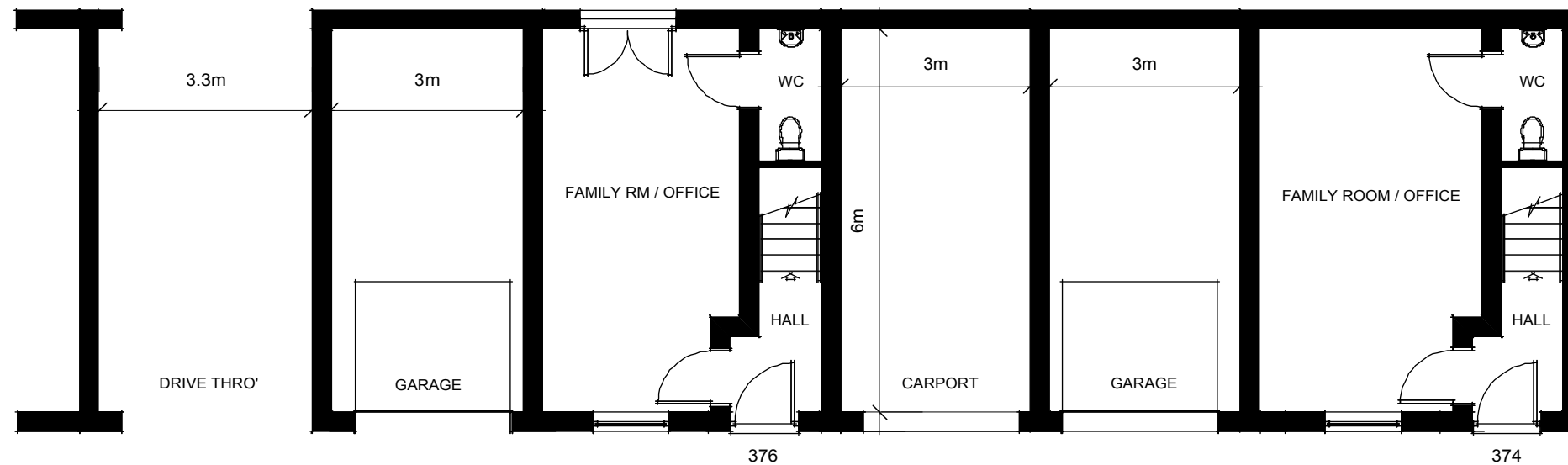
Ground Floor
