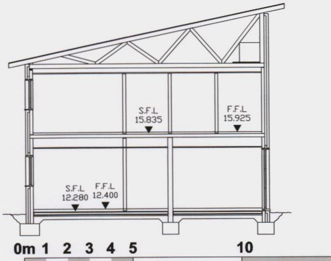
1:100 Layout existing section
