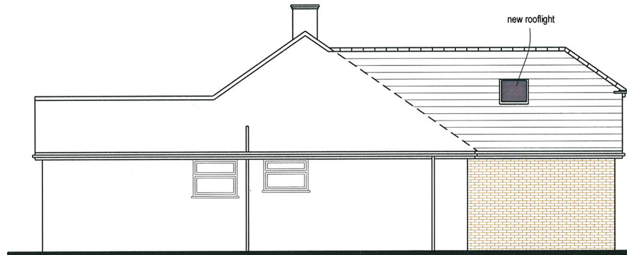
Proposed West Elevation (Side) 1:100
