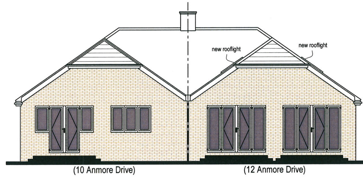
Proposed South Elevation (Rear) 1:100
