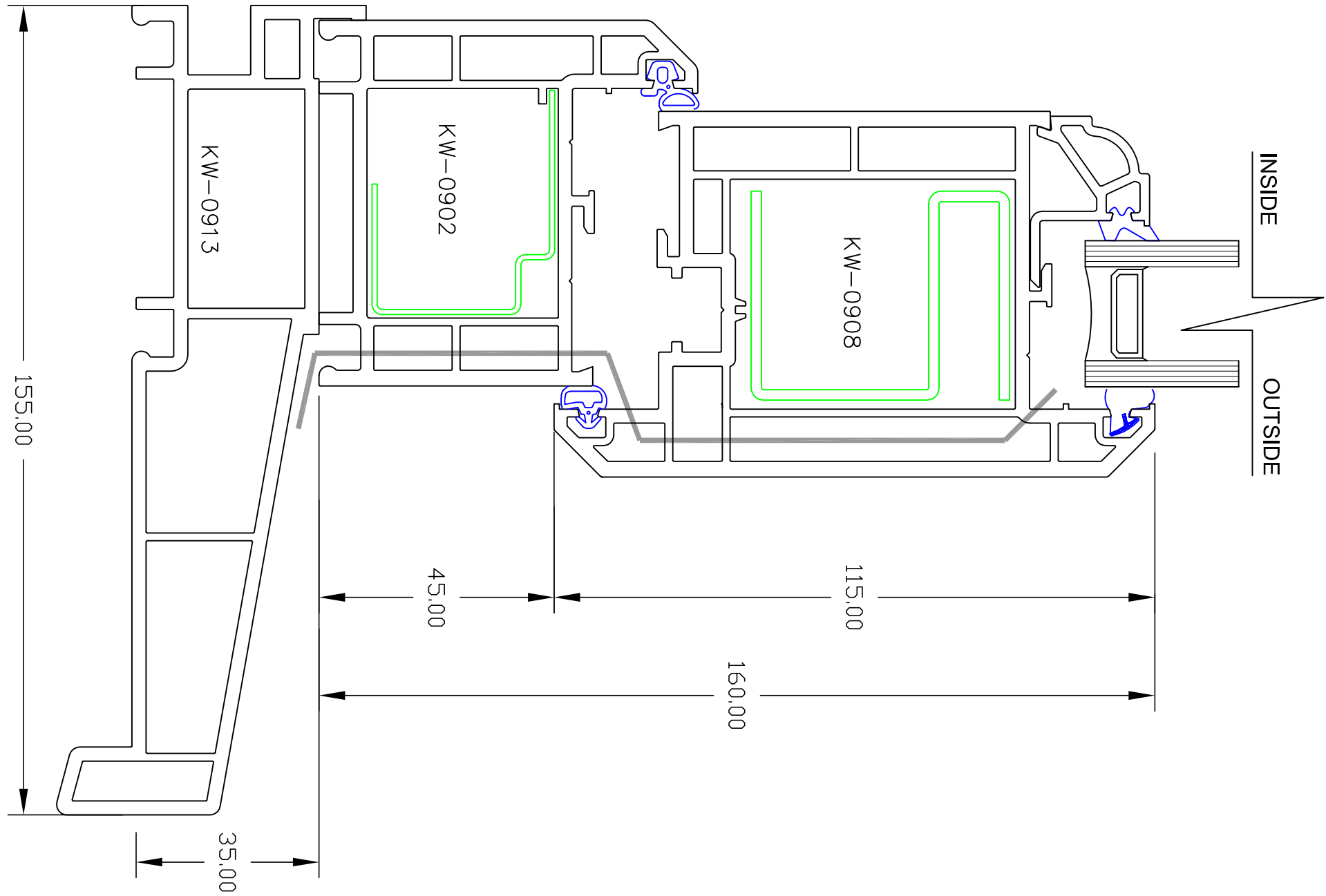
CILL TYPE A Opening out
