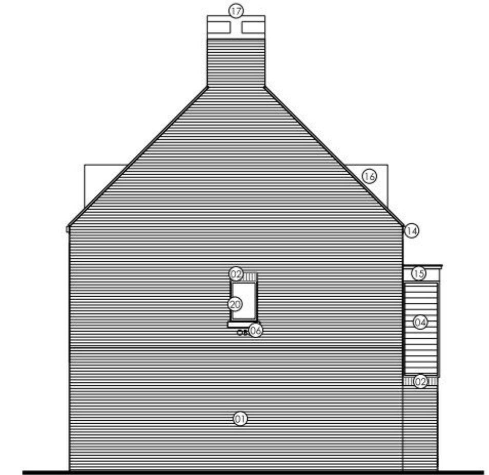
SIDE ELEVATION
