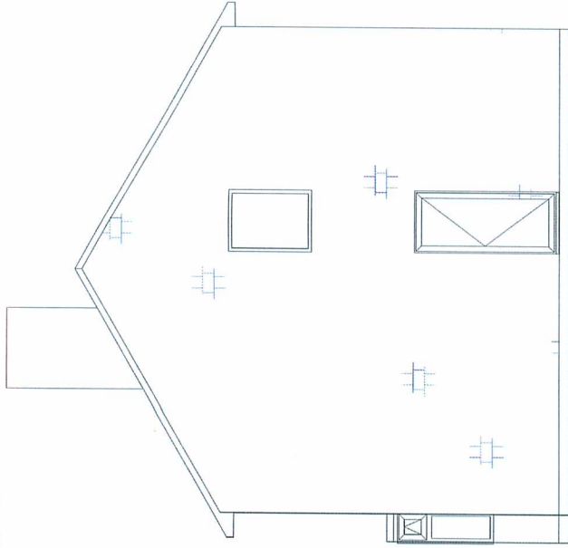
Existing Right Elevation
