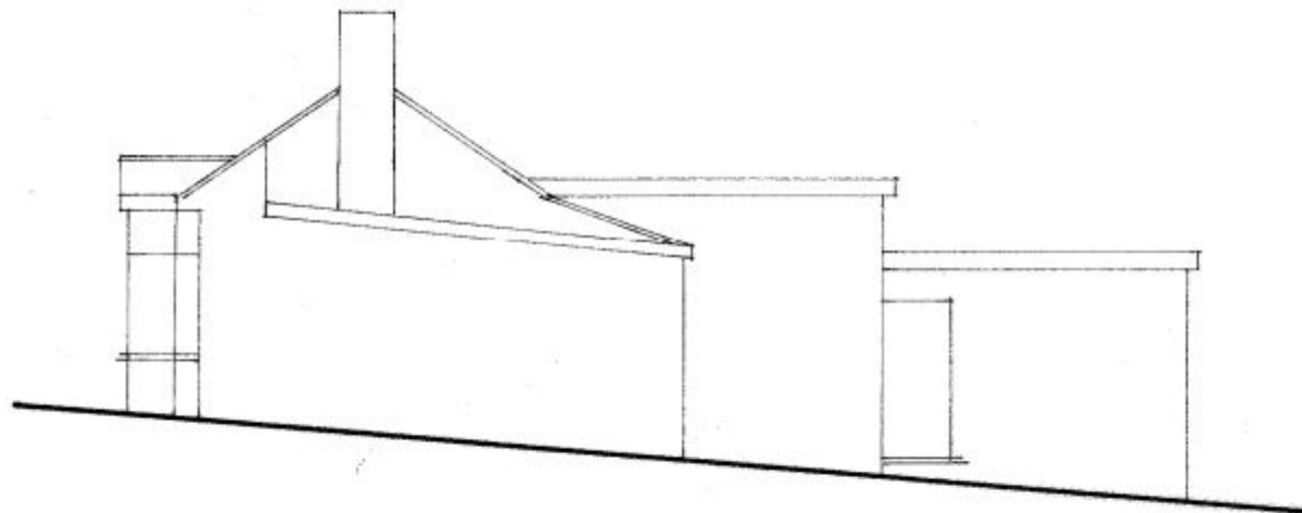
Existing East/Side Elevation
