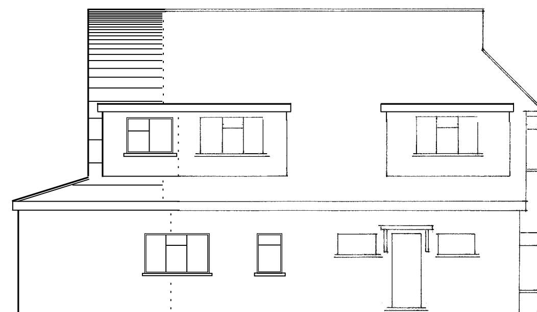
Proposed West/Side Elevation
