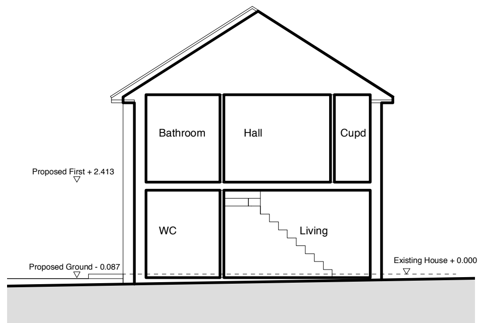
PROPOSED SECTION 1:100
