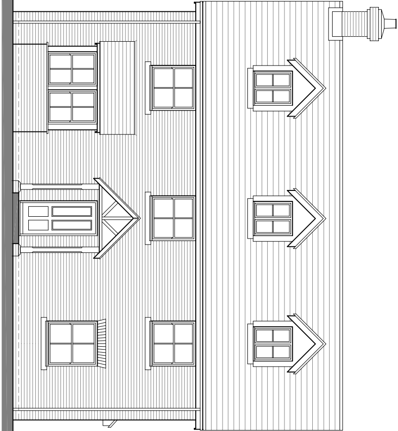
Front Elevation
