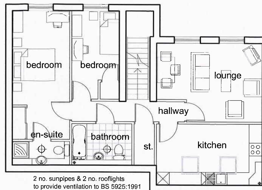
proposed first floor plan scale A1 1:50, A3 1:100
