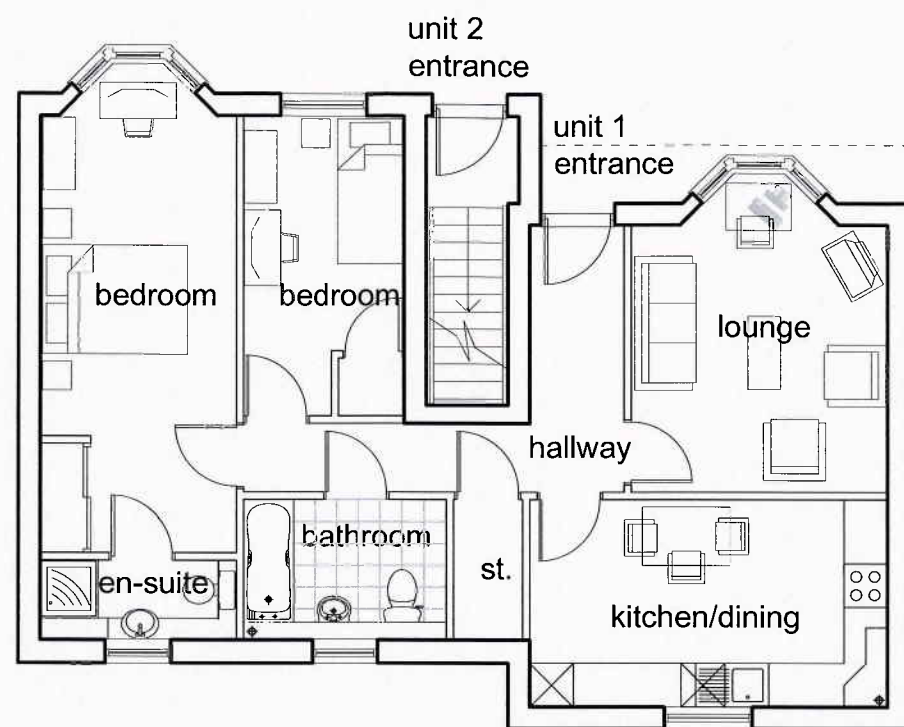
proposed ground floor plan scale A1 1:50, A3 1:100
