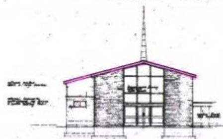
WEST ELEVATION
