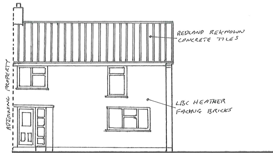
FRONT ELEVATION EXISTING
