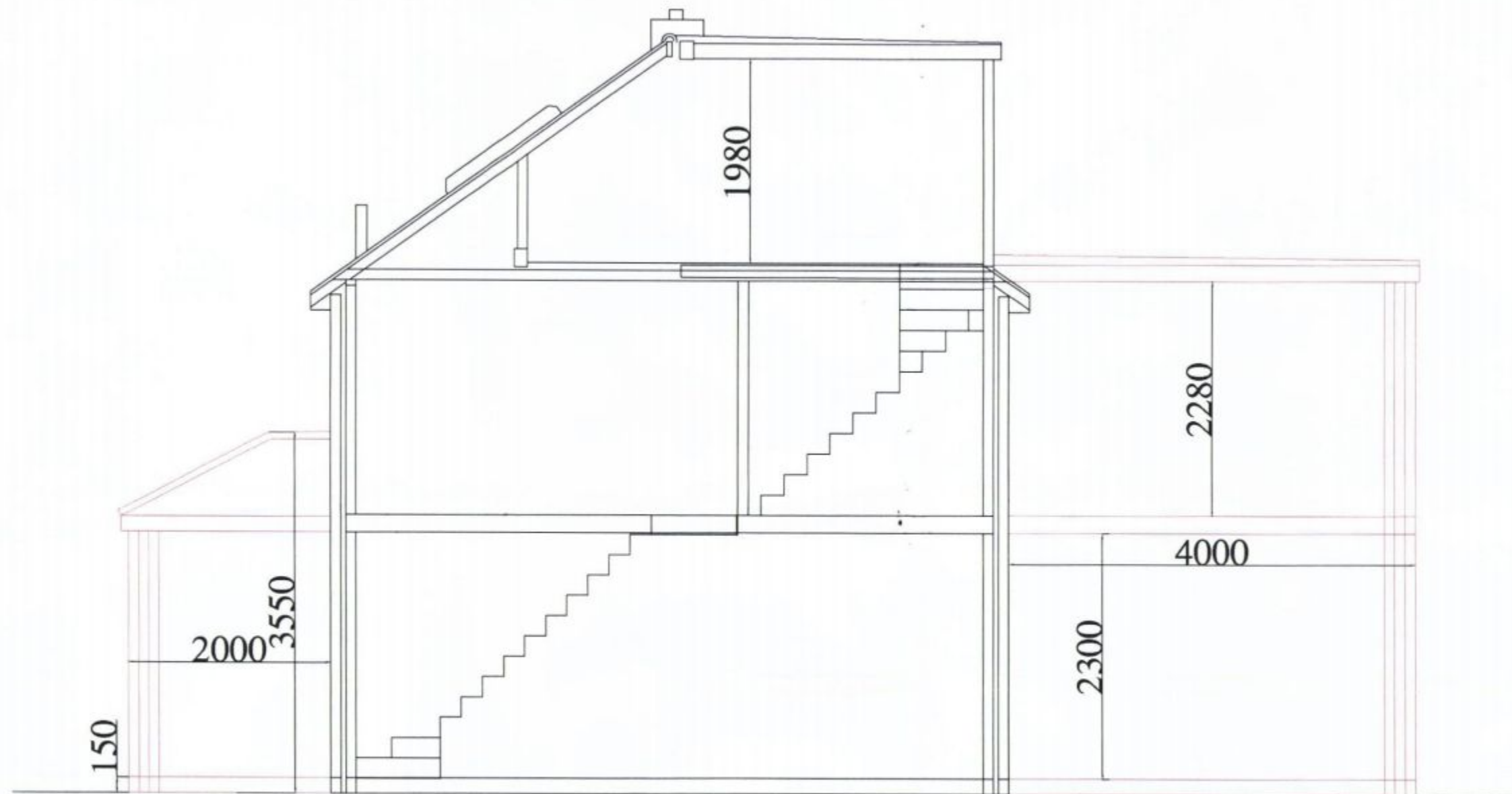
SECTION THROUGH SCALE 1:50
