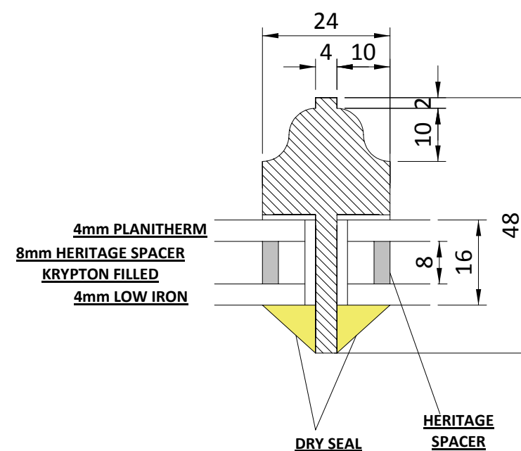
LAMBS TONGUE 10 X 10 PROFILE GLAZING BAR / HERITAGE SPACER DETAIL Scale 1 : 1 on A3
