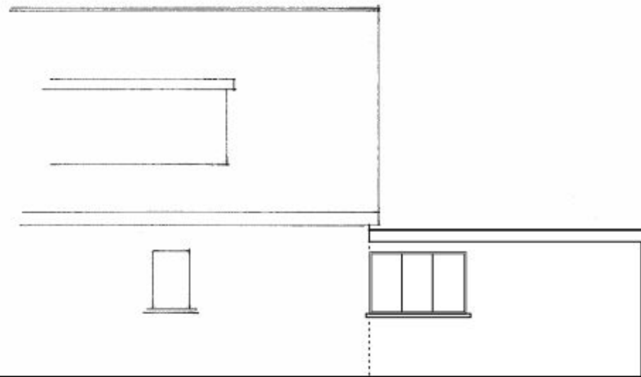
Proposed NE/Side Elevation
