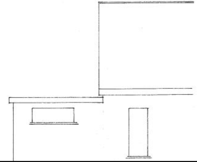
Existing SW/Side Elevation
