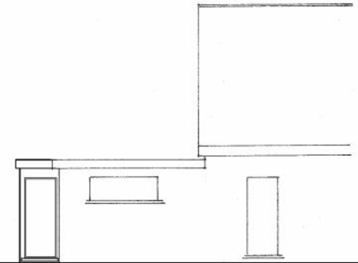
Proposed SW/Side Elevation
