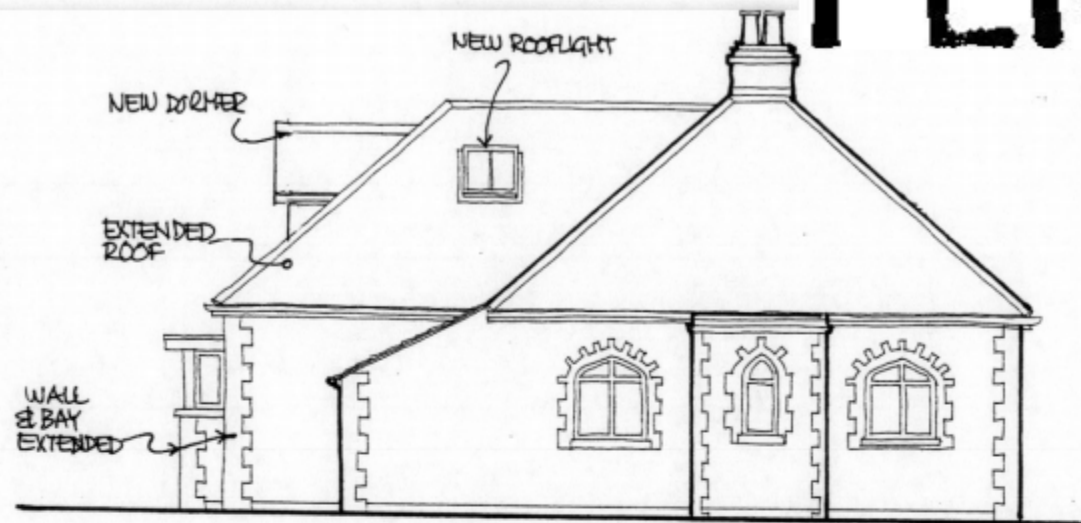
South Elevation (Ferry Road)
